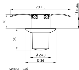
sensor head
