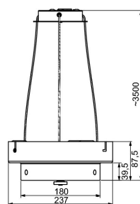
Maße [mm]
