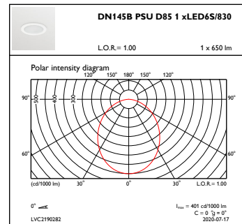
OFPC1_DN145BPSUD851xLED6S830
