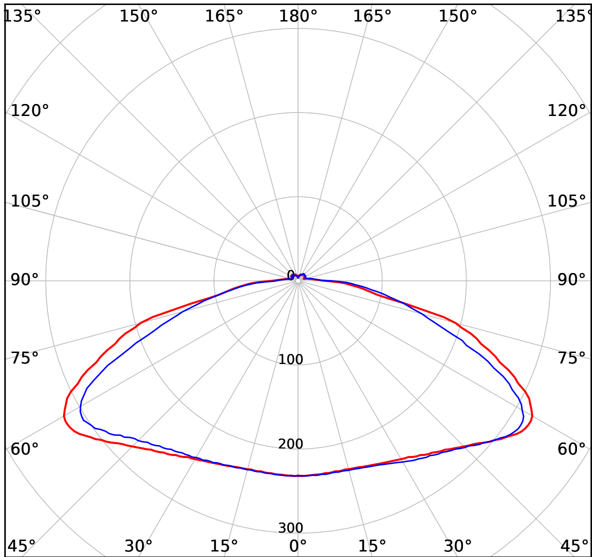
cd 1400 lm — C0-C180 — C90-C270
